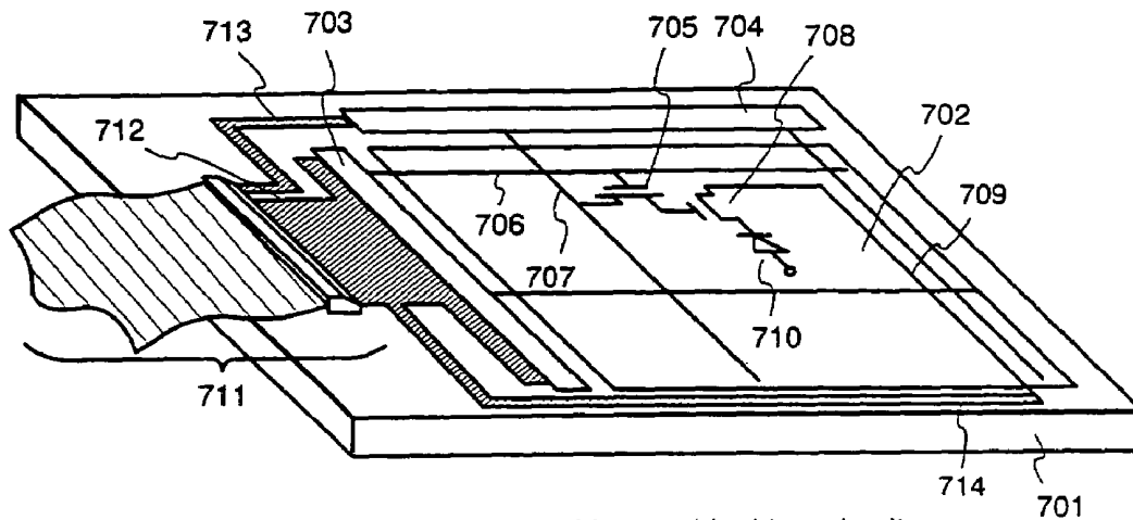
701:substrate 702:pixel portion 703:gate side driver circuit 704:source side driver circuit 705:switching TFT 706:gate wiring 707:source wiring 708:current control TFT 709:current supply line 710:EL element 711:FPC 712-714:connection wiring
